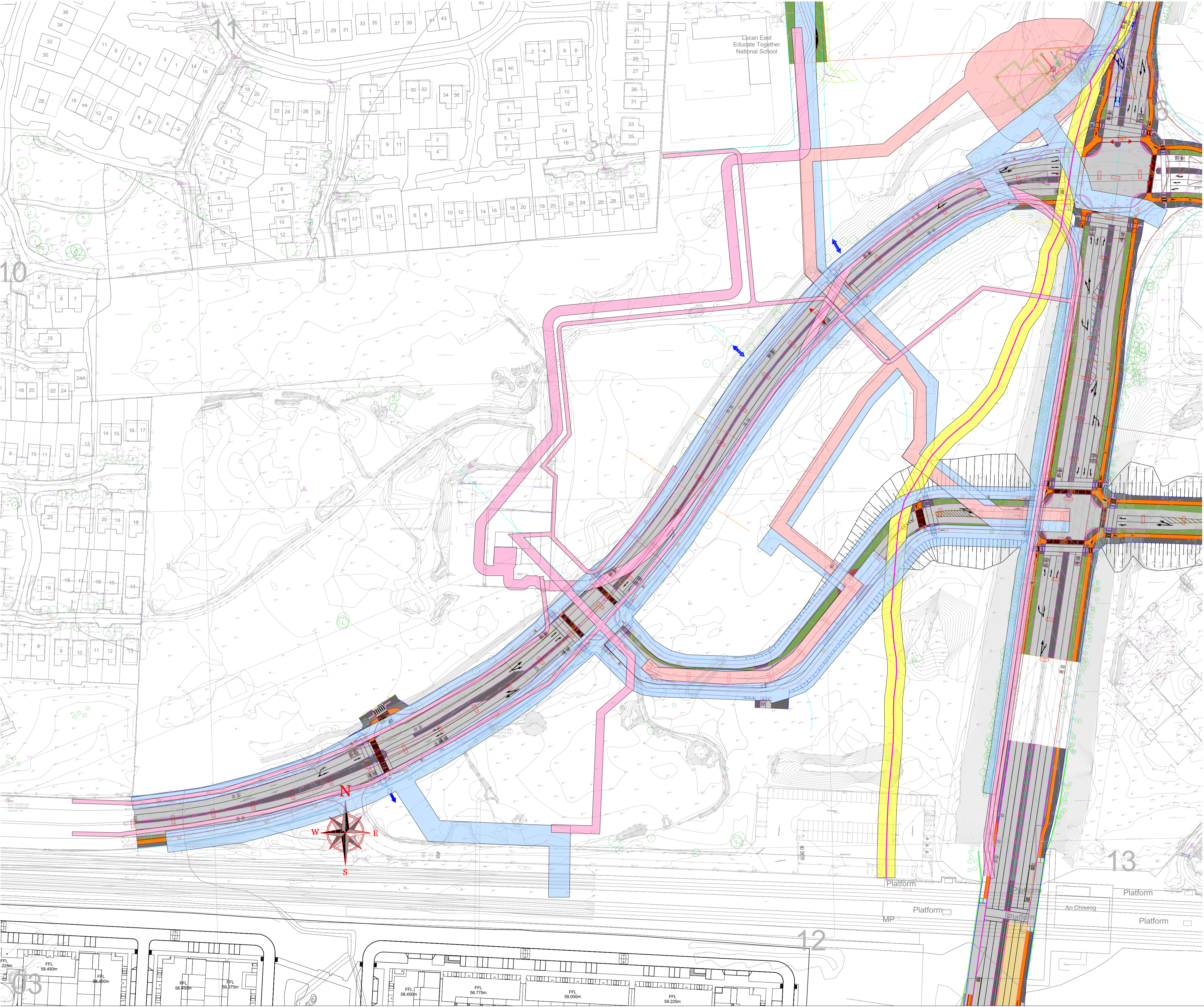
Site 3 Existing Realigned Services + Survey Layout
